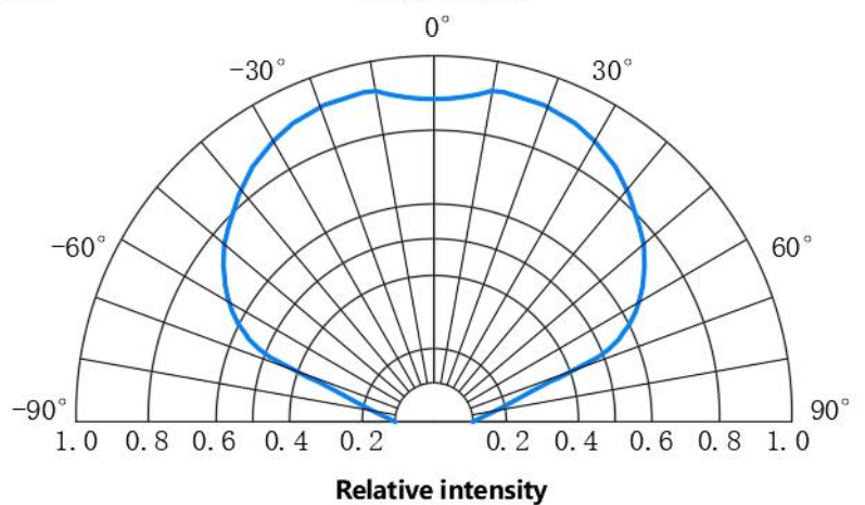
Beam Pattern
