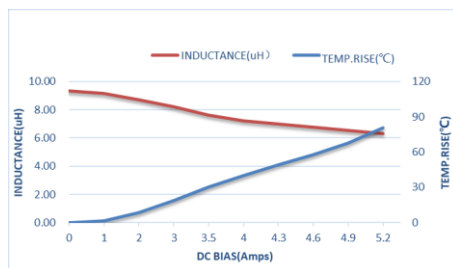
ZETC404020S100MGT-LF
