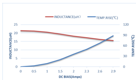
ZETC404020S220MGT-LF
