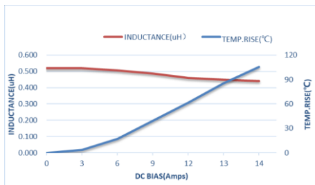
ZETC404020SR47MGT-LF
