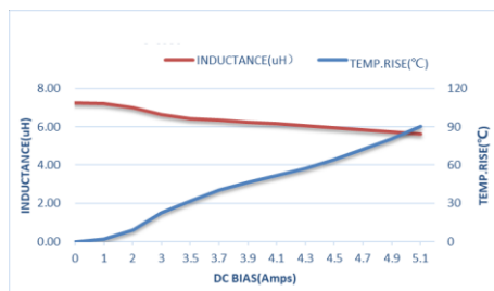
ZETC404020S6R8MGT-LF
