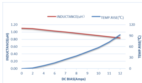
ZEMS404020-1R0M
