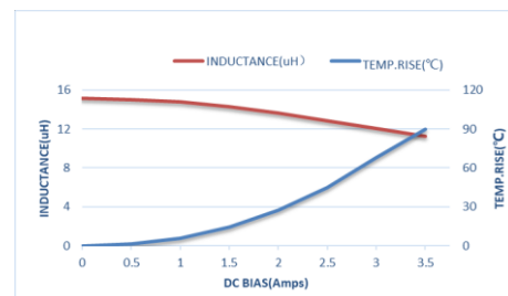
ZEMS404020-150M
