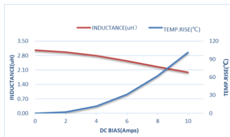
ZEMS404020-3R3M
