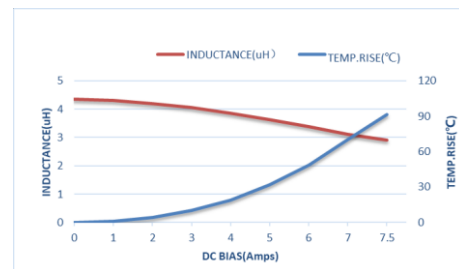
ZEMS404020-4R7M
