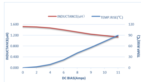
ZEMS404020-1R5M
