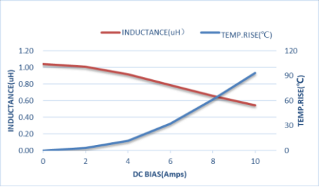
ZEPIM303012T1R0MLF
