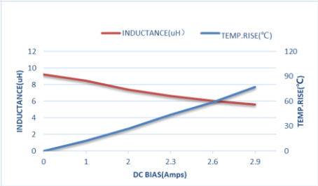
ZEPIM303012T100MLF
