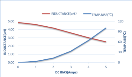
ZEPIM303012T4R7MLF
