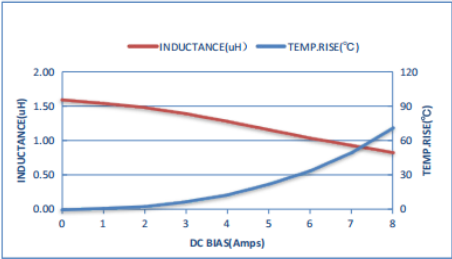
ZEPIM303012T1R5MLF
