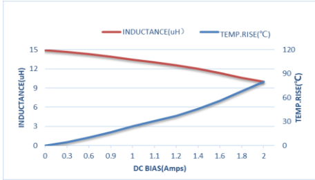
ZEPIM303012T150MLF
