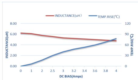
ZEPIM303020T6R8MLF
