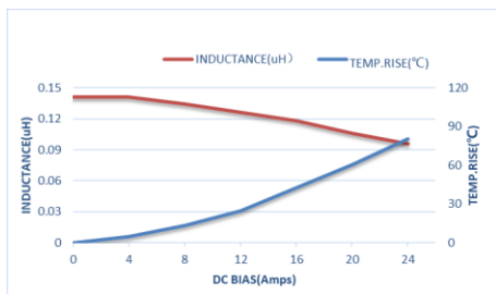
ZEPIM303020TR15MLF
