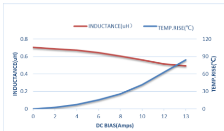
ZEPIM303020TR68MLF
