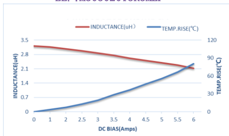
ZEPIM303020T3R3MLF
