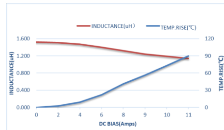
ZEMS404020-1R5M
