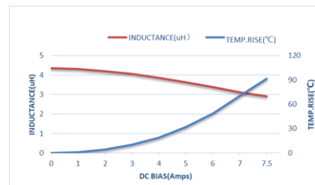
ZEMS404020-4R7M
