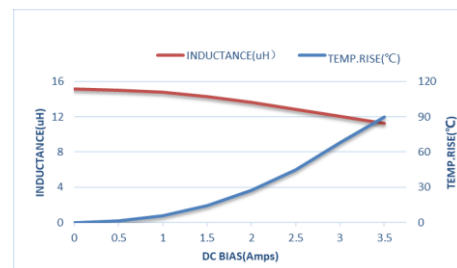
ZEMS404020-150M
