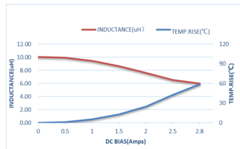
ZETC404010S-100MT-LF
