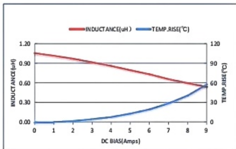
ZETC404010S-1R0MT-LF
