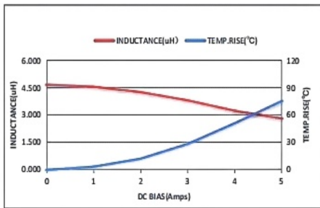
ZETC404010S-4R7MT-LF
