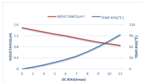
ZET-CORE-303020DT1R5MBCA
