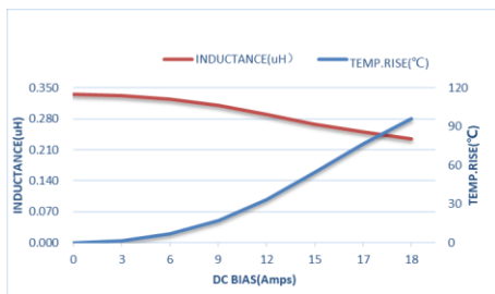
ZET-CORE-303020DTR33MBCA
