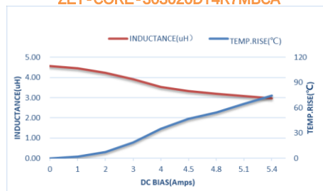
ZET-CORE-303020DT4R7MBCA
