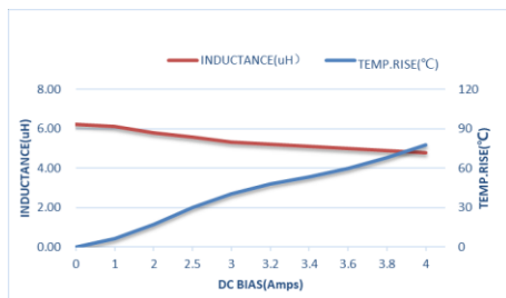
ZET-CORE-303020DT6R8MBCA
