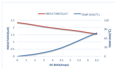
ZET-CORE-303020DT2R2MBCA
