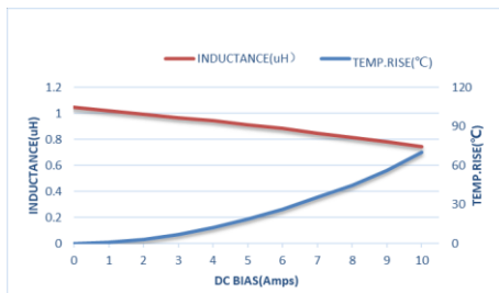
ZET-CORE-303020DT1R0MBCA
