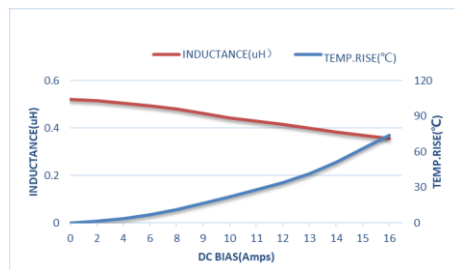
ZET-CORE-303020DTR50MBCA
