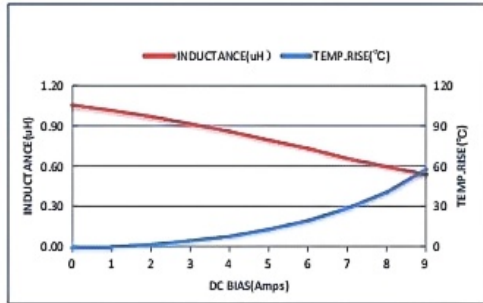
ZETC404010S1R0MBT-LF
