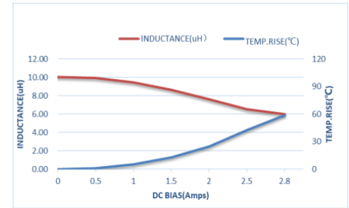
ZETC404010S100MBT-LF
