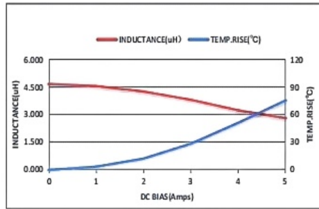
ZETC404010S4R7MBT-LF
