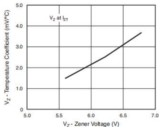
Figure 4: Temperature Coefficient
