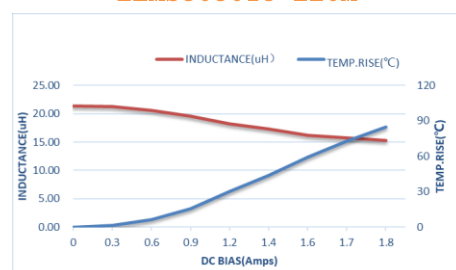
ZEMS303015-220M
