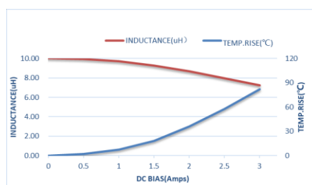
ZEMS303015-100M
