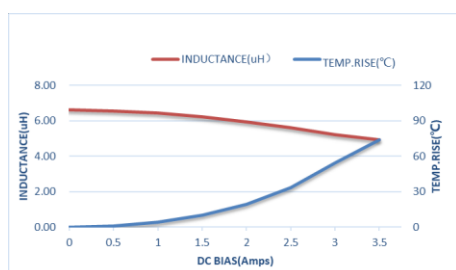
ZEMS303015-6R8M
