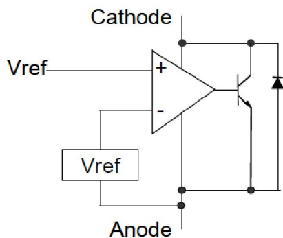
Figure 5 : Block diagram
