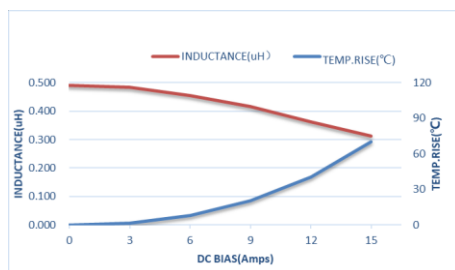
ZETC303018D-R47MT-LF
