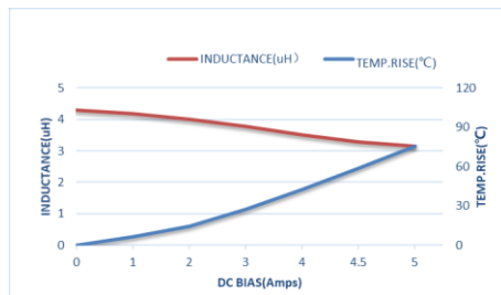
ZETC303018D-4R7MT-LF
