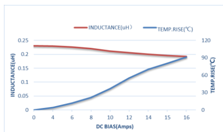
ZETC303018D-R22MT-LF
