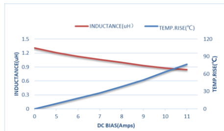
ZETC303018D-1R5MT-LF
