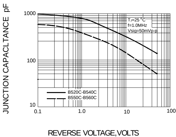
FIG.5-TYPICAL JUNCTION CAPACITANCE
