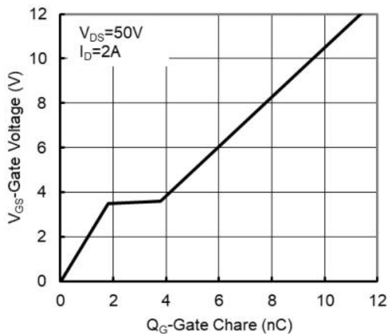
Figure 6: Gate-Charge Characteristics
