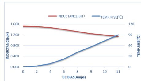
ZETC404020S1R5MGT-LF
