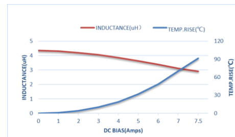
ZETC404020S4R7MGT-LF
