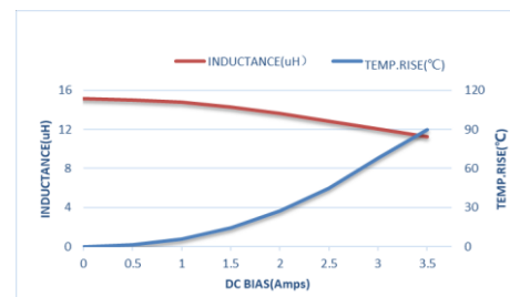
ZETC404020S150MGT-LF
