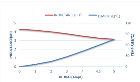
ZEPIM303018T4R7MLF
