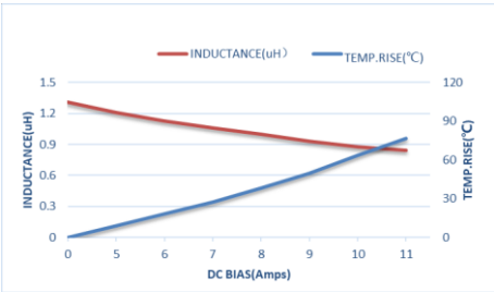
ZEPIM303018T1R5MLF
