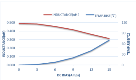
ZEPIM303018TR47MLF
