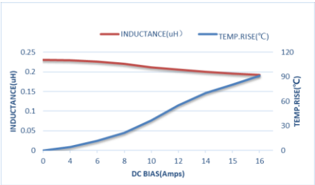
ZEPIM303018TR22MLF
