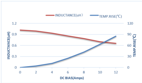
ZEPIM303018T1R0MLF
