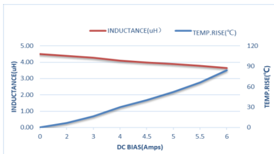
ZEMS404030-4R7M
