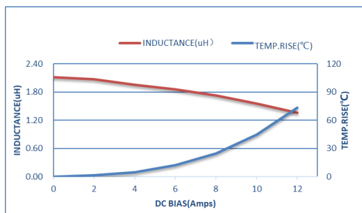
ZEMS404030-2R2M
