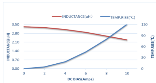
ZEMS404030-3R3M
