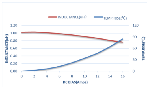
ZEMS404030-1R0M
