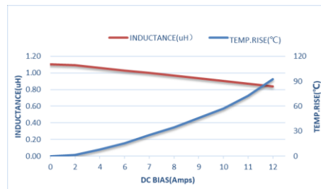
ZEP1M404020S-1R0M
