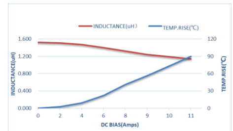
ZEP1M404020S-1R5M
