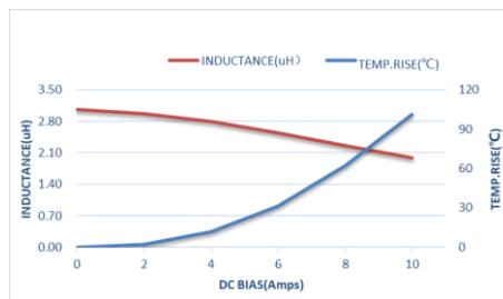
ZEP1M404020S-3R3M
