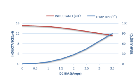
ZEP1M404020S-150M
