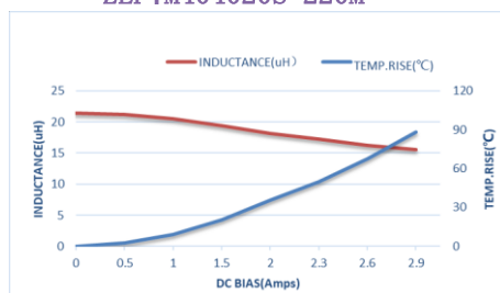
ZEP1M404020S-220M
