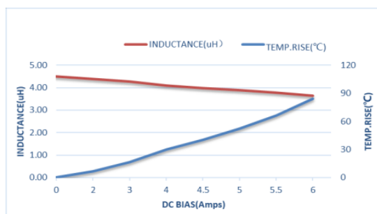
ZETC404030S-4R7MGT-LF
