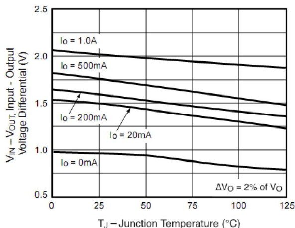
Figure 2. Dropout Voltage vs. Junction Temperature
