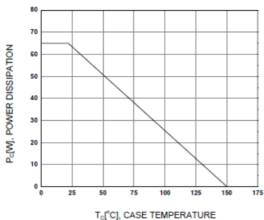
Figure 5. Power Derating
