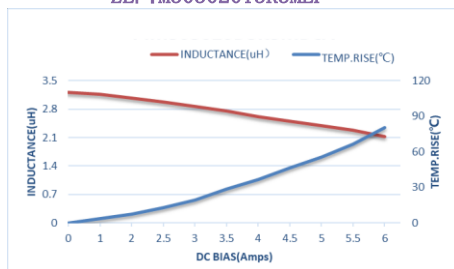
ZEPIM303020T3R3MLF
