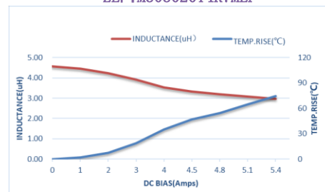
ZEPIM303020T4R7MLF
