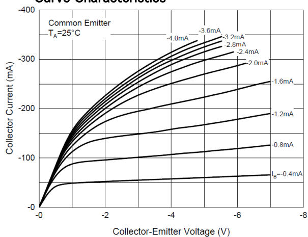
Static Characteristics
