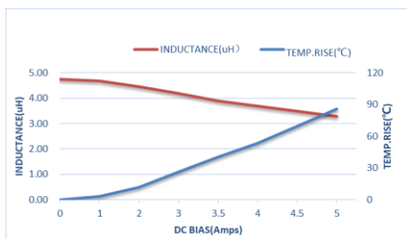
ZET-CORE-404012ST4R7MBCA
