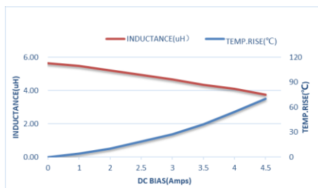
ZET-CORE-404012ST5R6MBCA
