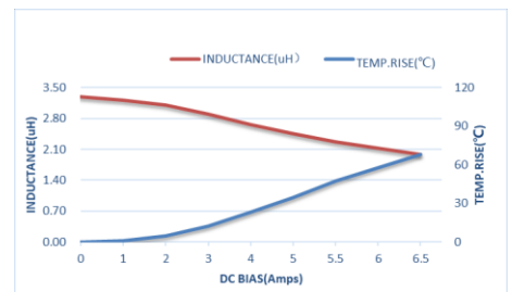
ZET-CORE-404012ST3R3MBCA
