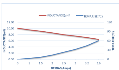
ZET-CORE-404012ST100MBCA
