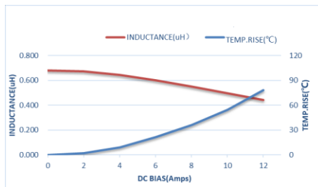
ZET-CORE-404012STR68MBCA
