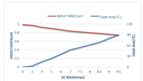
ZET-CORE-404012ST1R0MBCA
