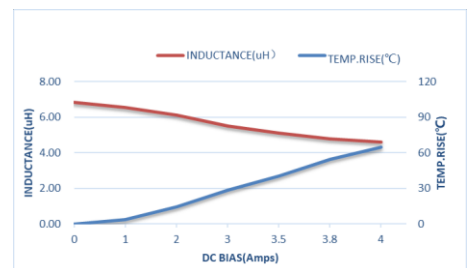
ZET-CORE-404012ST6R8MBCA
