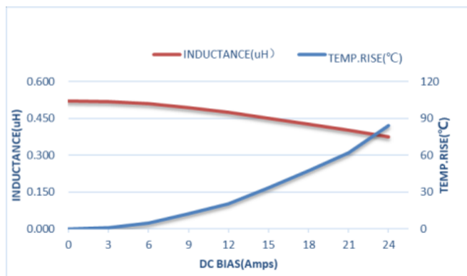
ZETC404030S-R47MT-LF
