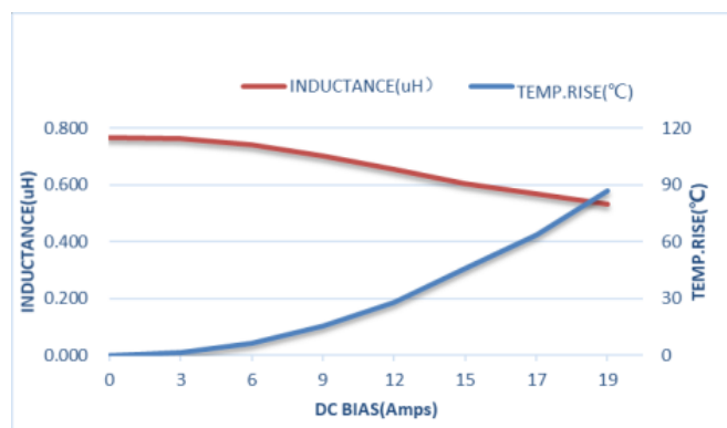
ZETC404030S-R68MT-LF
