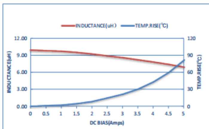
ZETC404030S-100MT-LF
