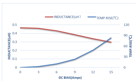
ZEMS303015-R47M
