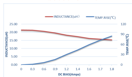
ZEMS303015-220M
