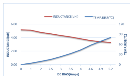
ZEMS303015-4R7M
