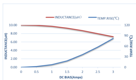
ZEMS303015-100M
