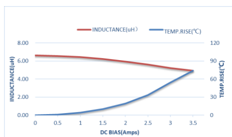
ZEMS303015-6R8M
