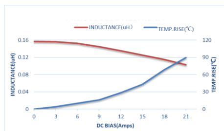
ZEMS303015-R15M
