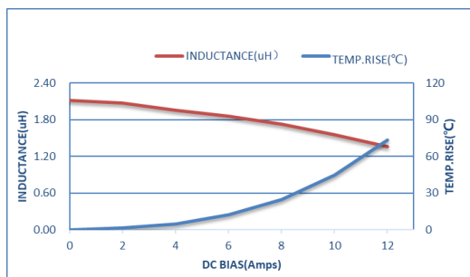
ZET-CORE-404030ST2R2MGCA
