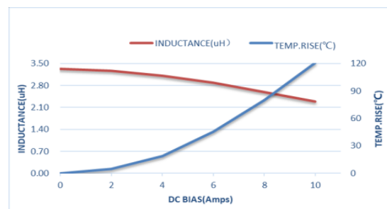
ZET-CORE-404030ST3R3MGCA
