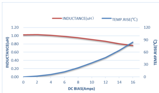
ZET-CORE-404030ST1R0MGCA
