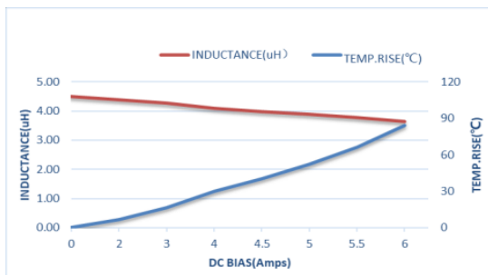
ZET-CORE-404030ST4R7MGCA
