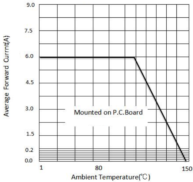
Fig 1-forwardCurrent derating Curve
