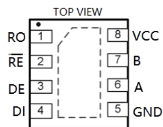
DFN-8 3*3
