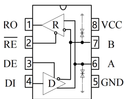
DIP-8/SOP-8/MSOP-8
