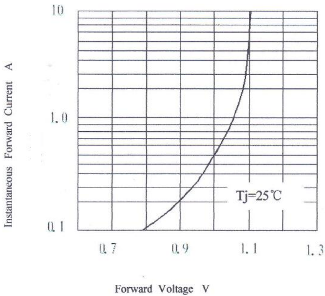
FIG4.Instantaneous Forward Voltage
