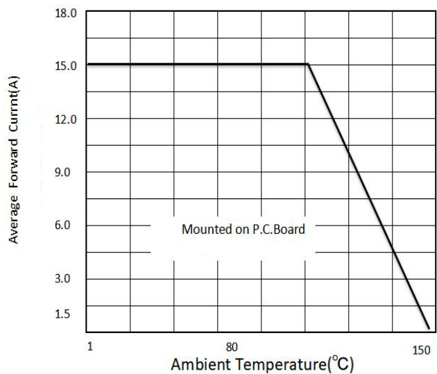
Fig 1-forwardCurrent derating Curve
