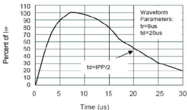
Pulse Waveform
