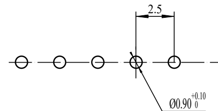
PCB LAYOUT
