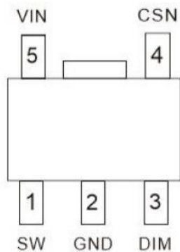
PT4115-TD(SOT89-5)
