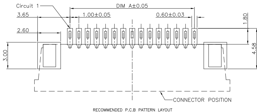
RECOMMENDED P.C.B. PATTERN LAYOUT
