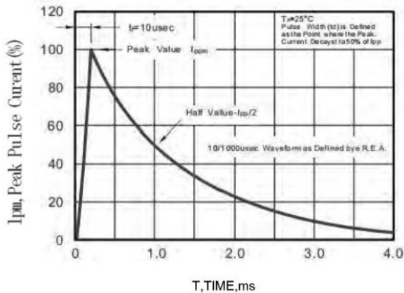
Fig.3 Pulse Waveform
