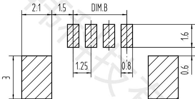
PCB LAYOUT
