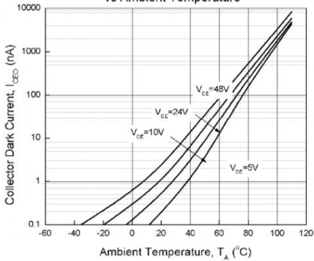
Figure 7. Collector Dark Current vs Ambient Temperature
