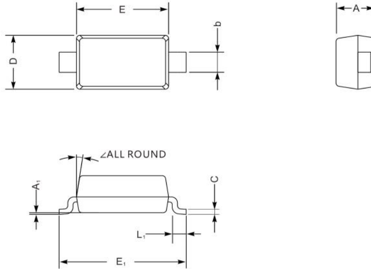
SOD-123 mechanical data
