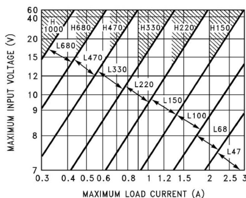
LM2576HV-5.0
