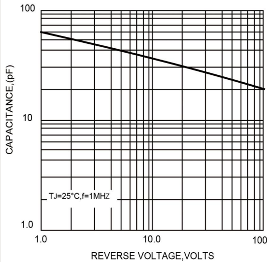
FIG.3-TYPICAL JUNCTION CAPACITANCE
