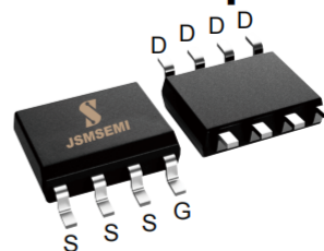
Top View of SOP-8
