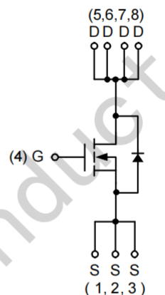
N-Channel MOSFET
