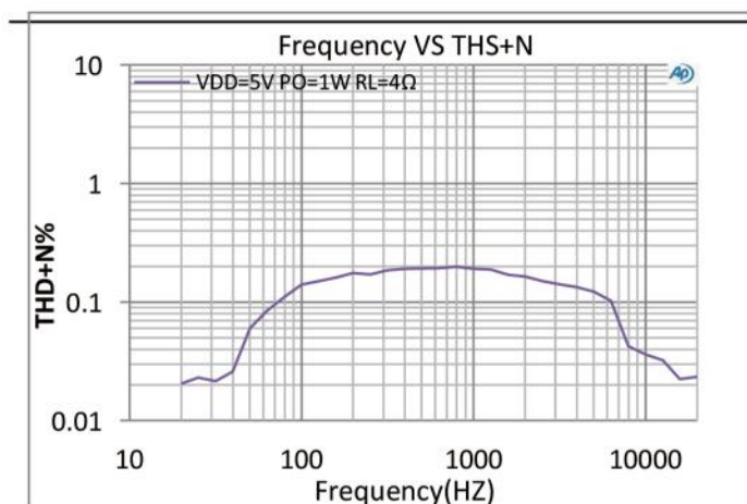
图5 : Frequency VS.THD+N
