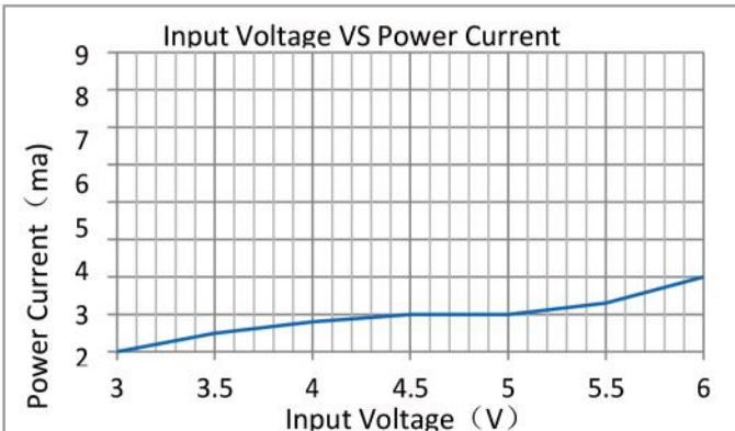
图4 : Input Voltage VS. Power Current
