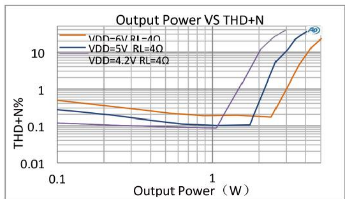
图3 : Output Power VS. THD+N
