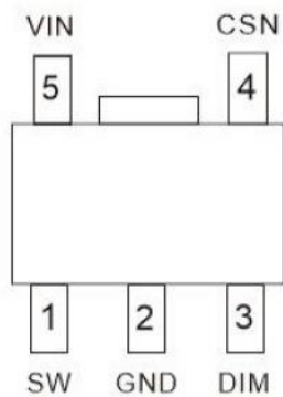
D3815C-TD(SOT89-5)
