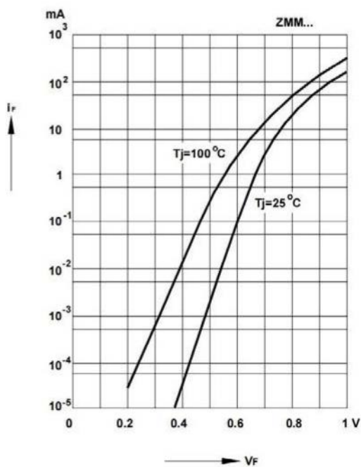
Forward characteristics
