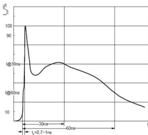
ESD pulse waveform according to IEC61000-4-2
