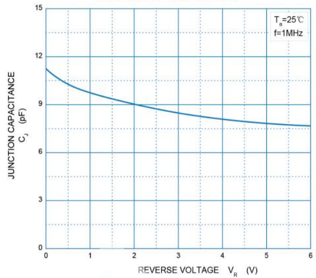
Capacitance Characteristics
