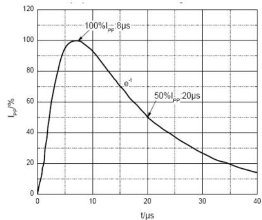
8/20 \mu\text{s} pulse waveform according to IEC 61000-4-5
