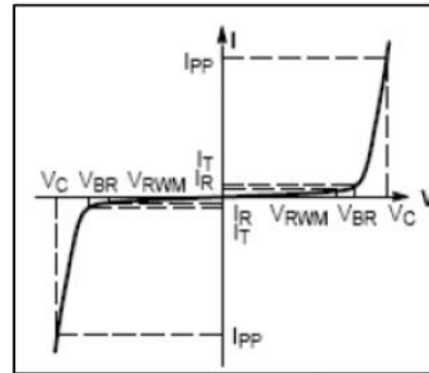
V-I characteristics for a Bi-directional TVS
