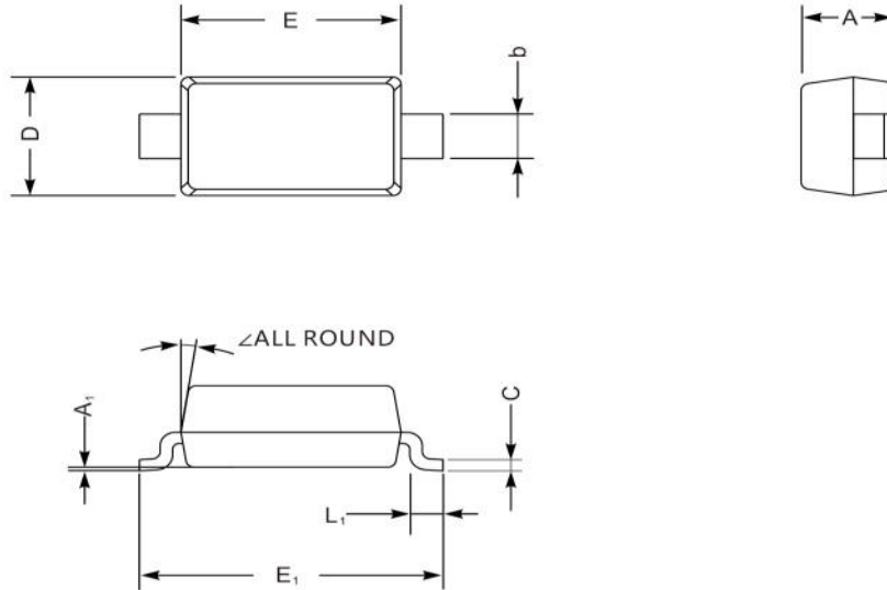
SOD-123 mechanical data
