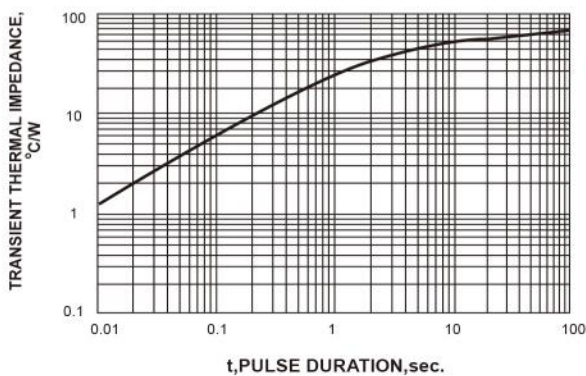
FIG. 5-TYPICAL TRANSIENT THERMAL IMPEDANCE
