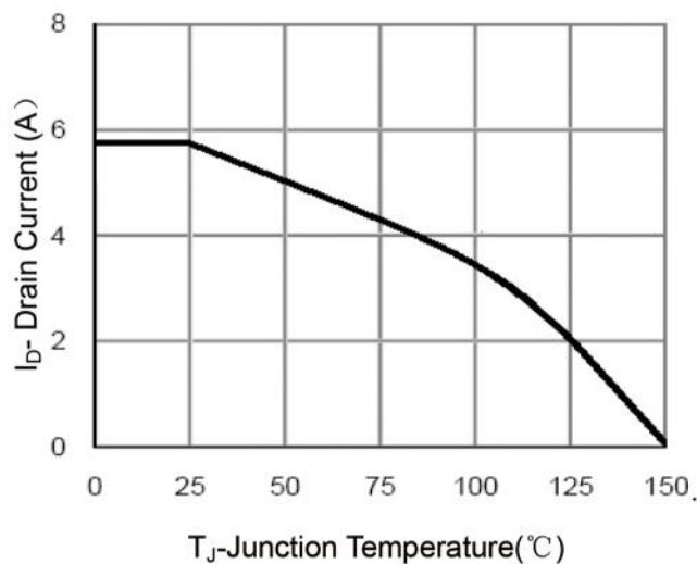
Figure 4 Drain Current
