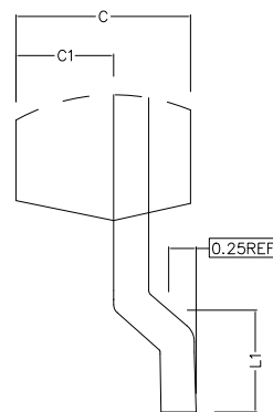
DETAIL E
